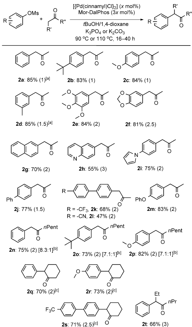
Scheme 3. Scope of the palladium-catalyzed \alpha -arylation of ketones with aryl mesylates. Reaction conditions: 0.6–0.8 mmol ArOMs, 5–10 equiv ketone, [\text{Pd}]/[\text{L}] = 2:3 , [\text{ArOMs}] = 0.5\text{--}0.125\text{ M} . See the Supporting Information. Yields are of isolated material, and mol% [\text{Pd}(\text{cinnamyl})\text{Cl}]_2 is indicated within parentheses. [a] Yield determined on the basis of calibrated GC data of 2a and 2d using dodecane as an internal standard. [b] Mixture of regioisomers. Ratio indicated within brackets, with major product shown. [c] Used tert -butanol solvent, \text{K}_2\text{CO}_3 , 110^\circ\text{C} .
